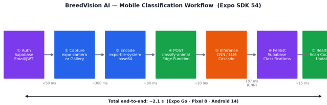
Fig. 4: Mobile flowchart for Expo SDK 54: Auth → Capture → Encode → POST → Inference → Persist → Realtime Update. Total end-to-end: \approx 2.1 s on Pixel 8, Android 14 [19].
