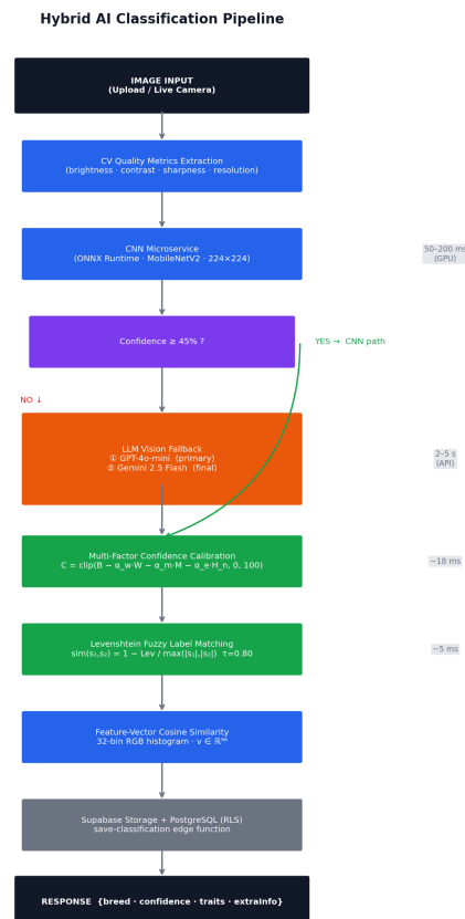
Fig. 1: Pipeline Architecture for Hybrid AI Classification: input images undergo inference using the CNN CNN main inference, LLM cascading for low confidence, multiple criteria calibration, Levenshtein fuzzy matching, and Supabase historical data storage. Timing markers indicated below right.
