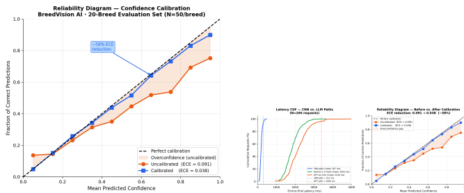
(a) Reliability diagram: uncalibrated (ECE=0.091) vs. calibrated (ECE=0.038). Shaded area = overconfidence gap. (b) Left: Latency CDF — CNN path (blue, 187ms mean) vs. LLM paths (orange/green). Right: Reliability diagram.
