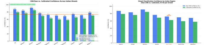
(a) Raw CNN vs. calibrated confidence across ten breeds. Orange dashed line: mean calibrated accuracy (73.8%).
